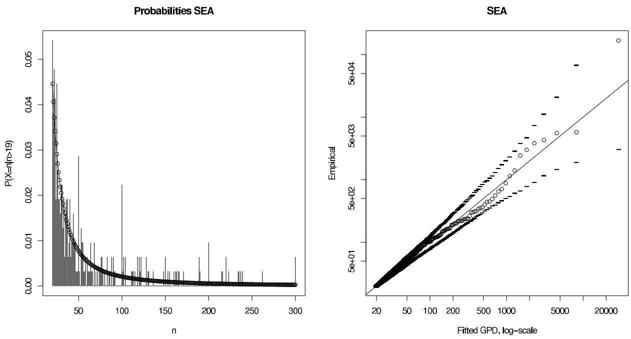
Figure 2: Empirical probabilities, fitted DGPD and QQ-plot SEA, at least 20 dead.
