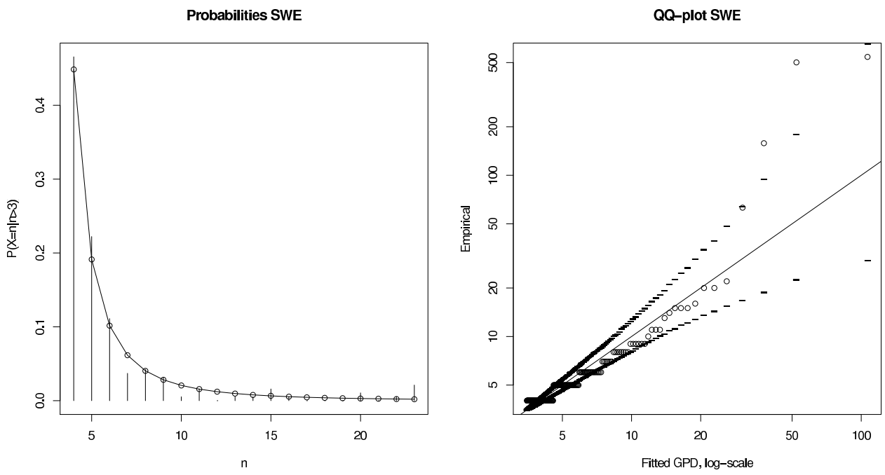
Figure 3: Empirical probabilities, fitted DGPD and QQ-plot SWE, at least four dead.
