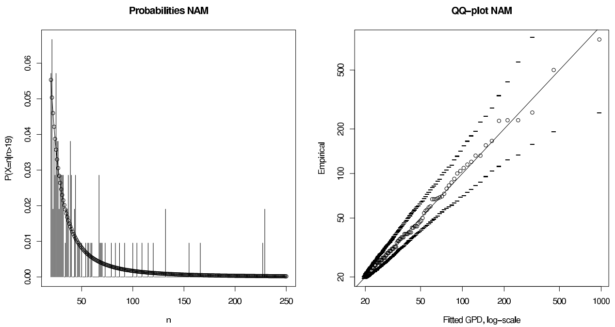
Figure 1: Empirical probabilities, fitted DGPD and QQ-plot NAM, at least 20 dead.
