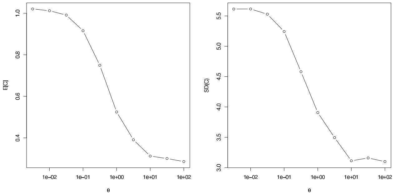
Figure 5: E[C] and SD(C) as functions of \theta
