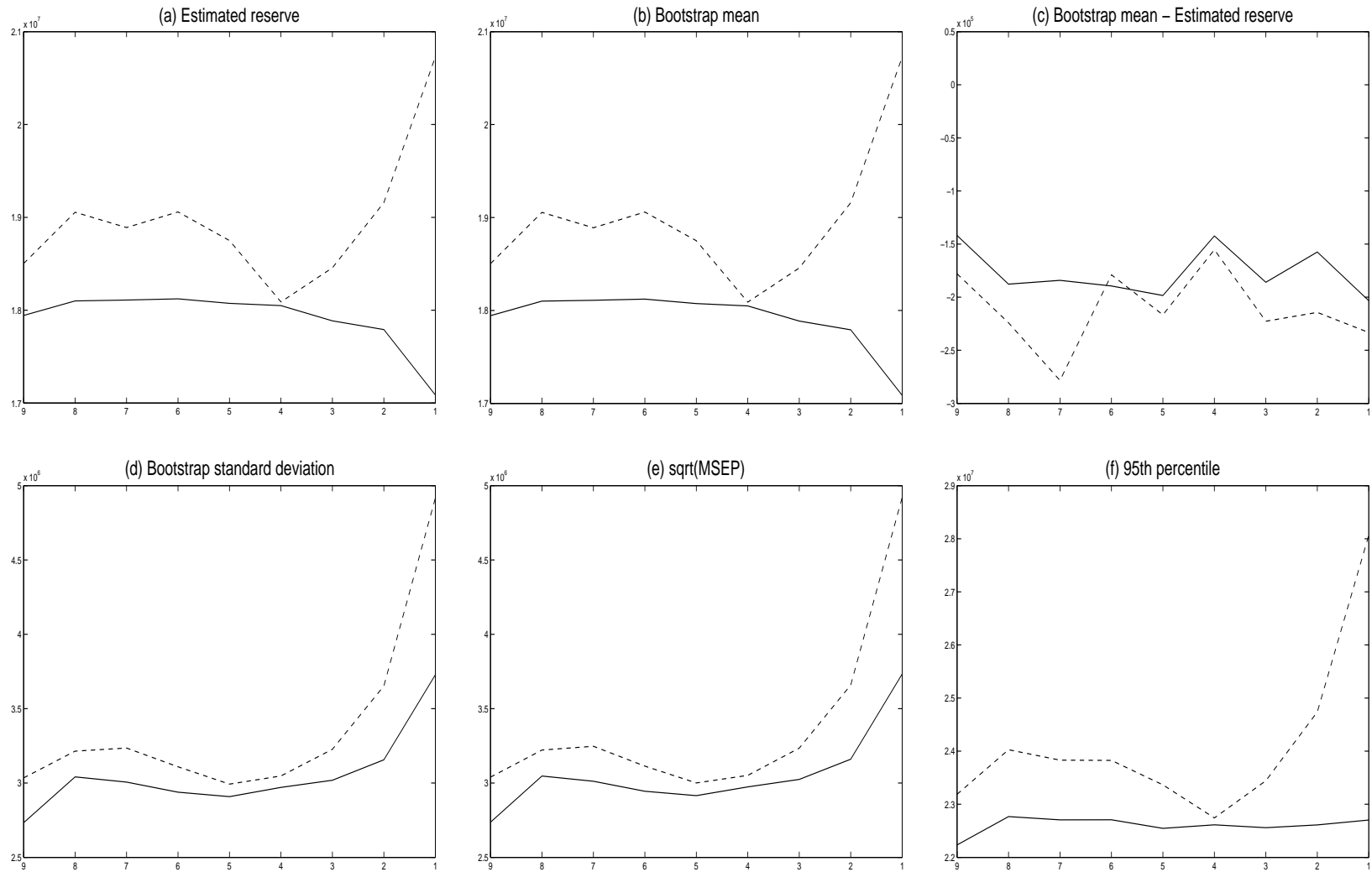
Figure 3: Reserve estimates and bootstrap statistics for the assumption of an ODP and a gamma distribution, respectively. Here we use (- - -) for the ODP distribution and (-) for the gamma distribution. On the x -axis we have r .
