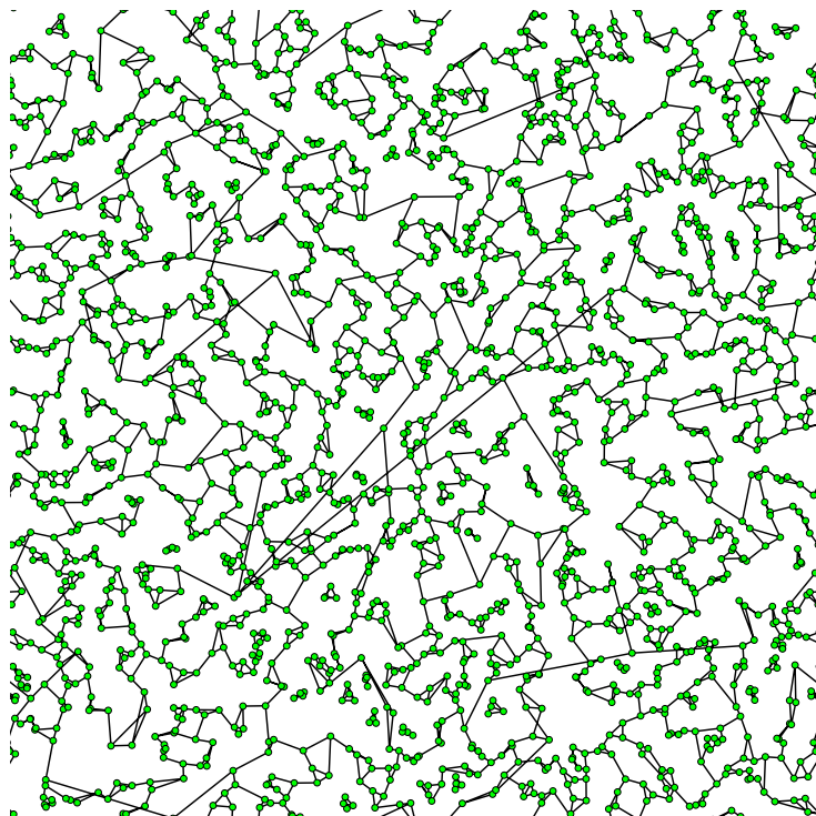
(b) \mathbb{P}(D = 3) = 1
