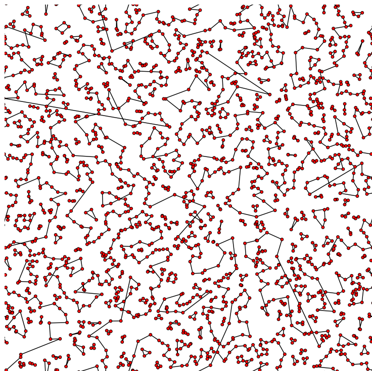
(b) \mathbb{P}(D = 2) = 1
