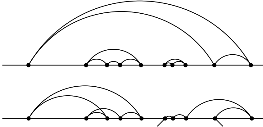
Figure 1: The stable multi-matching (top) and the random-direction stable multi-matching, for 10 vertices on a finite interval, with 2 stubs per vertex.
