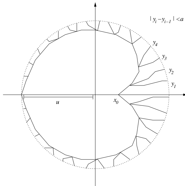
(b) The branches hit \partial B(0, u) at points \{y_i\} .
