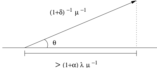
Figure 1: Choice of \theta .
